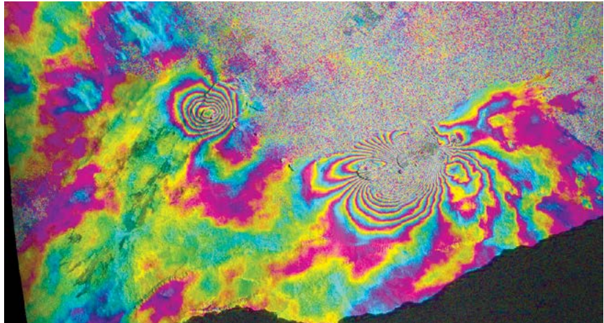
Figure 4. Relative deformation of Earth's surface at Kilauea between Feb. 11, 2011 and March 7, 2011 – two days following the start of the eruption on March 5, 2011 – imaged by radar interferometry using COSMO-SkyMed. Fringes mirror surface motion with 1.5 cm steps. Left: the circular pattern of concentric fringes represents deflation of the magma source beneath Kilauea. Right: the pattern represents the deformation caused by volcanic dike intrusion and subsequent fissure eruption taking place (P. Lundgren, NASA - JPL).
