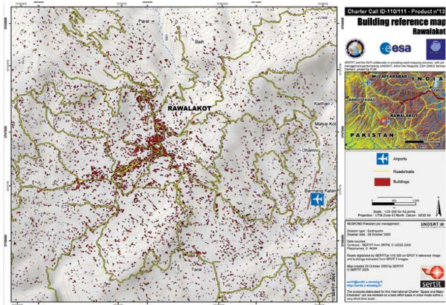
Figure 10. Extract from an asset mapping product by SERTIT in Pakistan, following the 8 October 2005 Asian earthquake, using SRTM DEM for contours and SPOT-5 data for road networks and built-up areas. Source: International Charter Space & Major Disasters and GMES Respond (ESA).
