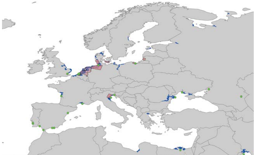
Figure 10. Europe, coastal lowlands (dark blue) and available PSI datasets concerning the coastal lowland subsidence and flood defence products of Terrafirma or SubCoast in orange and red (data derived from Terrafirma, www.terrafirma.eu.com and SubCoast, www.subcoast.eu ).
