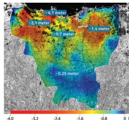
Figure 13. Land subsidence in Jakarta during the period 1974-2010, based on PSI (ERS-2 1996-1998, Envisat 2007-2009 and ALOS PALSAR 2007-2010), levelling, GPS, extensometers and groundwater level measurements. Source: Deltares 2011.
