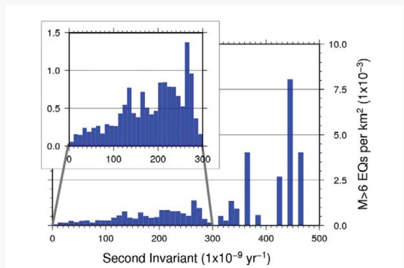
Figure 2. Number of earthquakes per square kilometre ( M > 6 from the ISC catalogue 1964-2010) as a function of the magnitude of tectonic strain (second invariant of strain tensor from Kreemer et al. (2003)).
