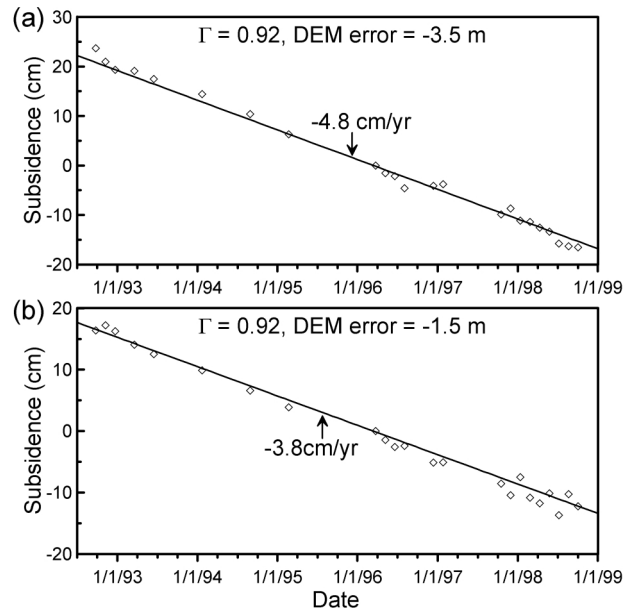
Fig. 8. Time series of elevation change at two selected PS points A (a) and B (b), whose locations are shown in Fig. 6. Estimated mean velocities are -4.8 cm/yr and -3.8 cm/yr in (a) and (b). Temporal coherence and DEM error estimated during PSInSAR processing are presented in the plots.
